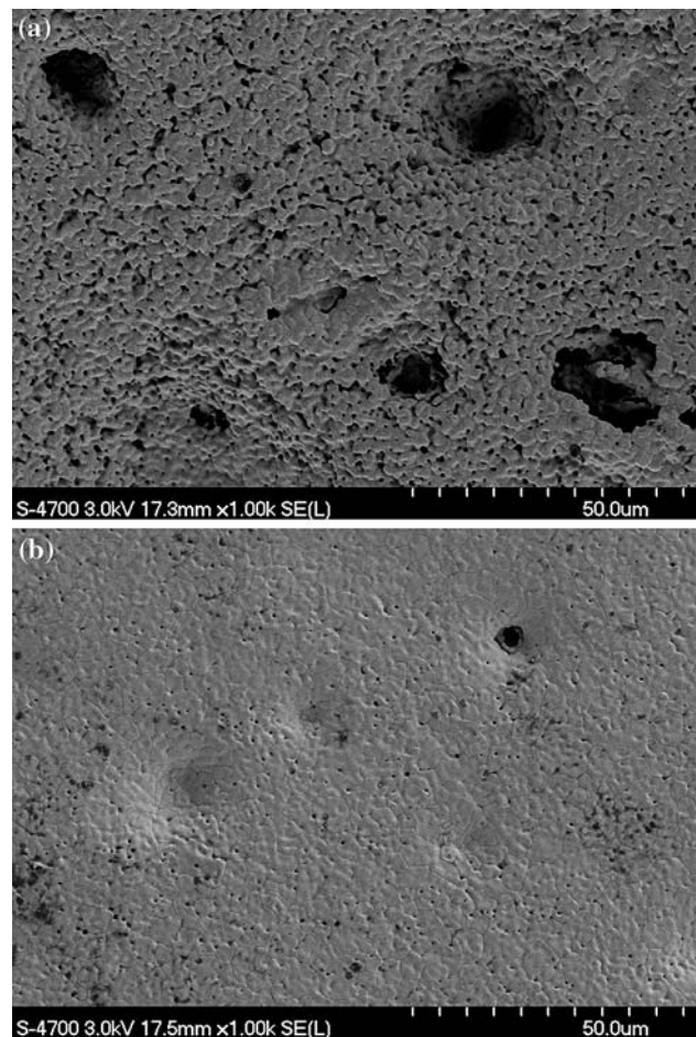
Fig. 14 SEM micrographs of different surfaces of a tape with 17.6 vol.% starch sintered at 1600 °C: a top surface, b bottom surface
