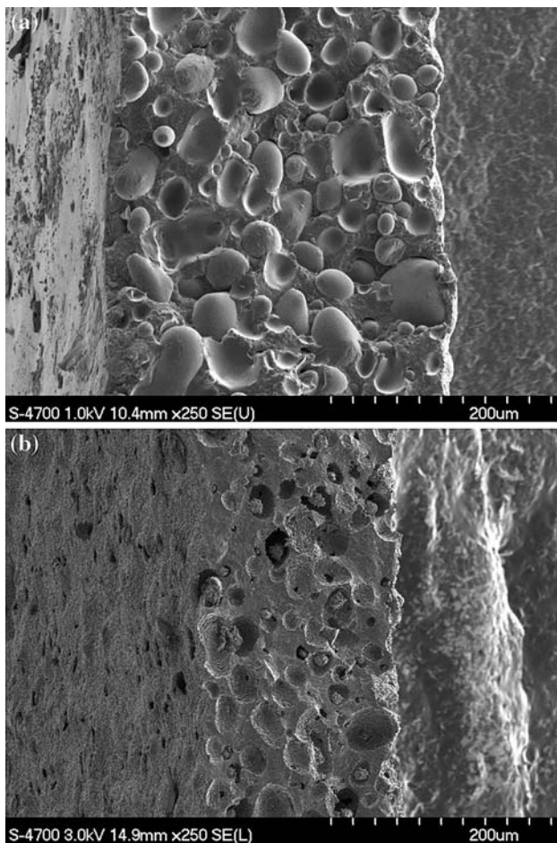
Fig. 13 SEM micrographs of a a green tape with 37.8 vol.% starch, b a tape with 37.8 vol.% starch sintered at 1600 °C
