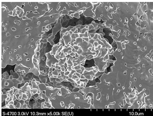
Fig. 12 SEM micrograph of a large pore with the inner YSZ shell for a tape with 37.8 vol.% starch sintered at 1500 °C
